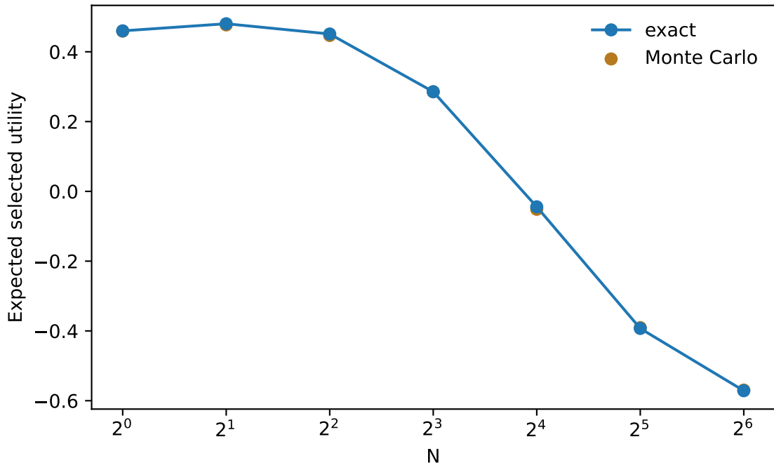
Finite-N law under tail misalignment
