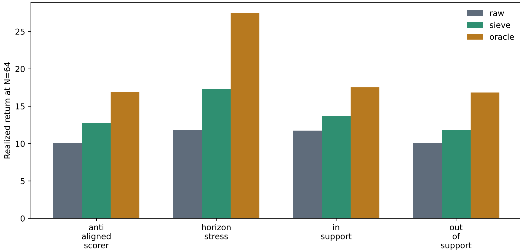
Support-Calibrated Plan Sieve versus raw Best-of-N
