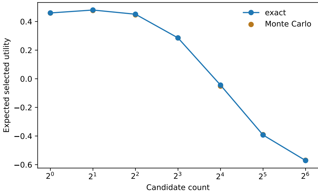
Finite-candidate identity under tail misalignment
