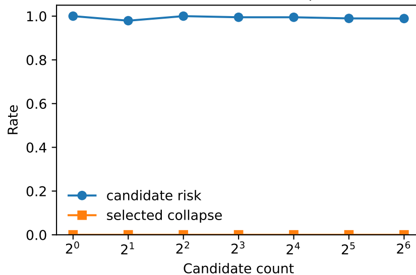
Search risk and collapse
