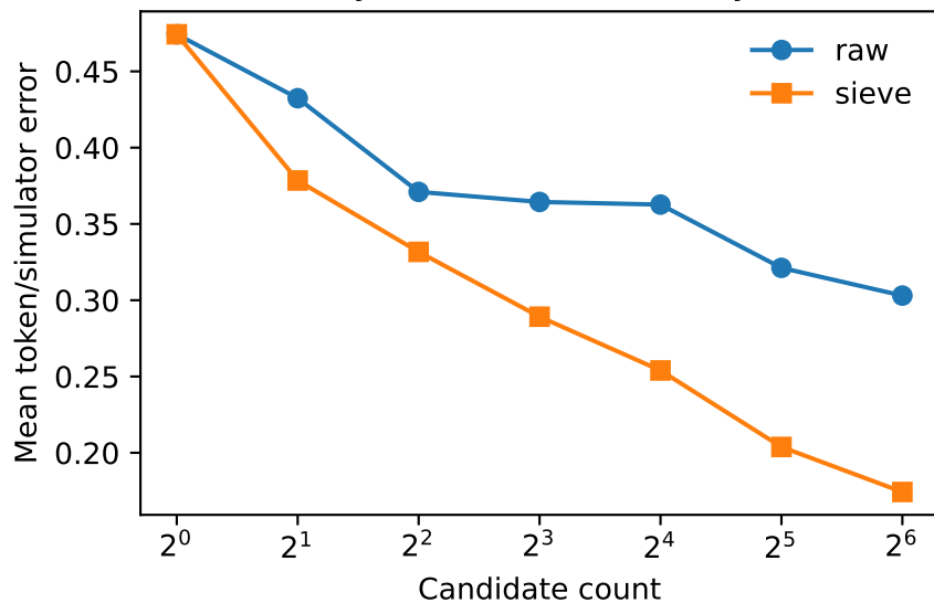
Dynamics inconsistency
