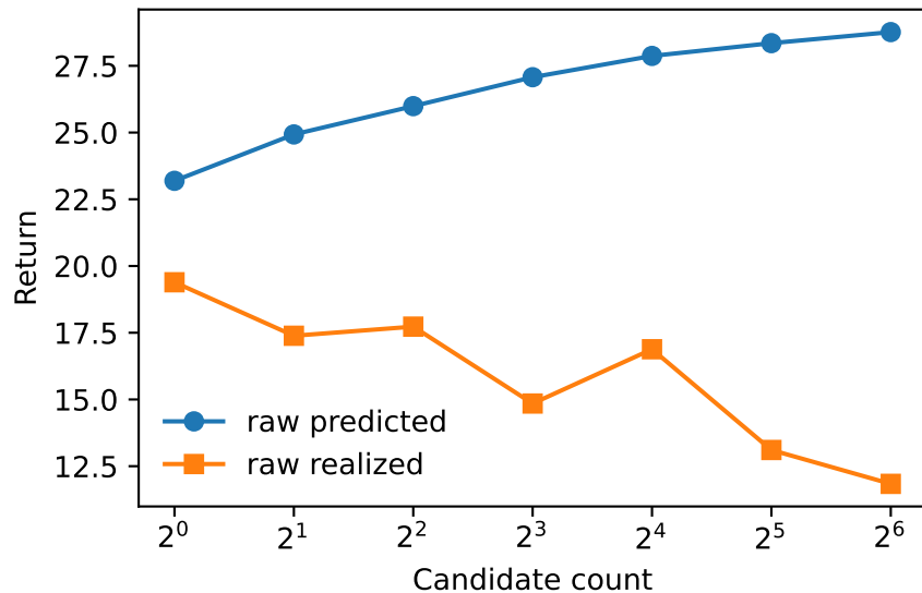
Reward-token extremization
