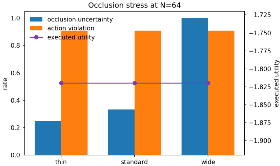
Figure 6: Occlusion stress from results/experiment_occlusion_stress.json . Wider occlusion increases uncertainty while large candidate-count raw visual selection continues to choose the invalid direct action family.
