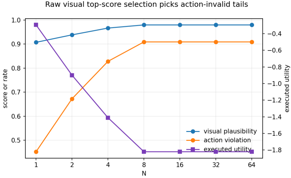
Figure 2: Failure metrics from results/experiment_video_tail_failure.json . Higher N improves the internal visual selection score while increasing action inconsistency and reducing real executed utility.
