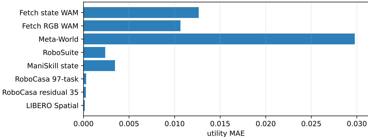
Exact-law utility MAE across rollout-pool artifacts
