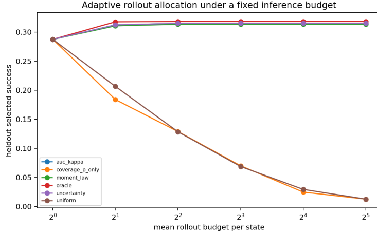
Figure 5: Inference-value profiles support adaptive rollout budgets. A moment-based allocator uses estimated marginal gains and avoids spending large budgets on states whose selection curves have saturated or become unhelpful. The result is an empirical budgeting diagnostic, not a universal controller theorem.
