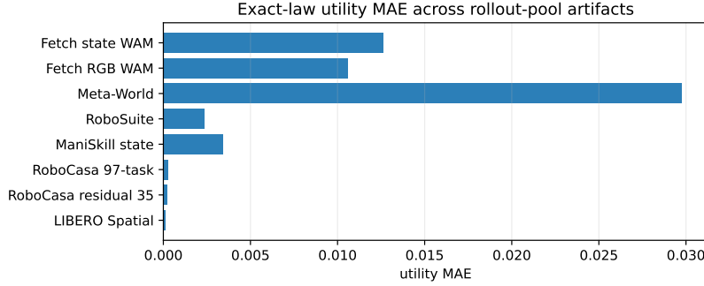
Figure 5: Exact-law error ledger. The finite tied-pool identity remains low-error across analytic, learned, visual, and simulator rollout-pool artifacts.
