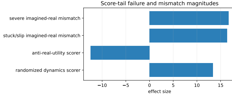
Figure 7: Failure-mode ledger. The same score-tail audit detects imagined-real mismatch, anti-real-utility scoring, and randomized-dynamics scoring failures.
