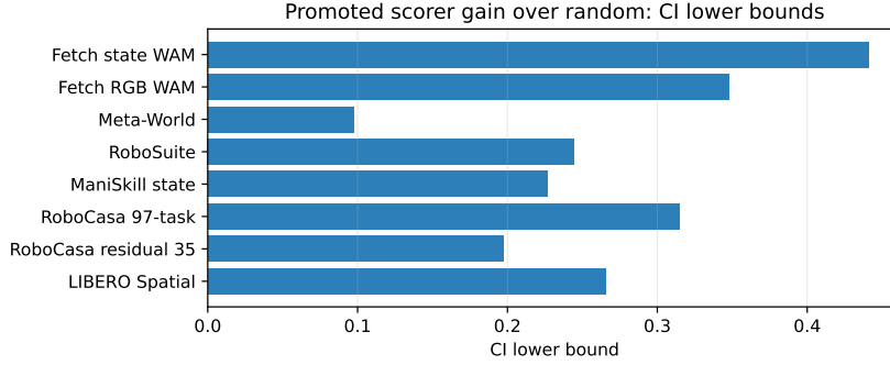
Figure 6: Promoted scorer gains over random. The v3 ledger reports CI lower bounds for the promoted learned or dense scorer in each benchmark family; negative or weak settings remain scoped as limitations.
