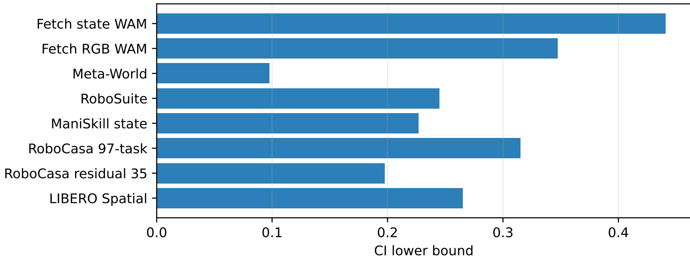
Promoted scorer gain over random: CI lower bounds
