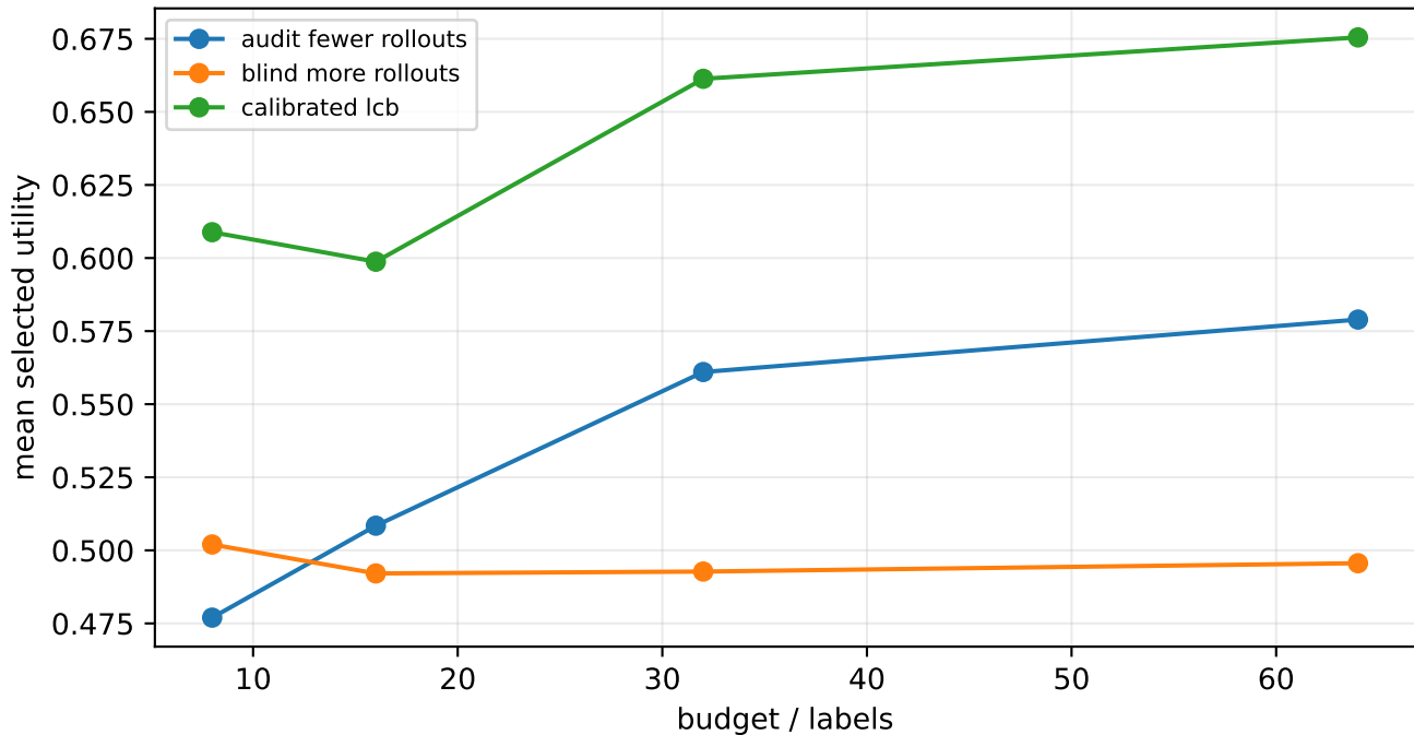
V5 equal-compute CPU frontier
