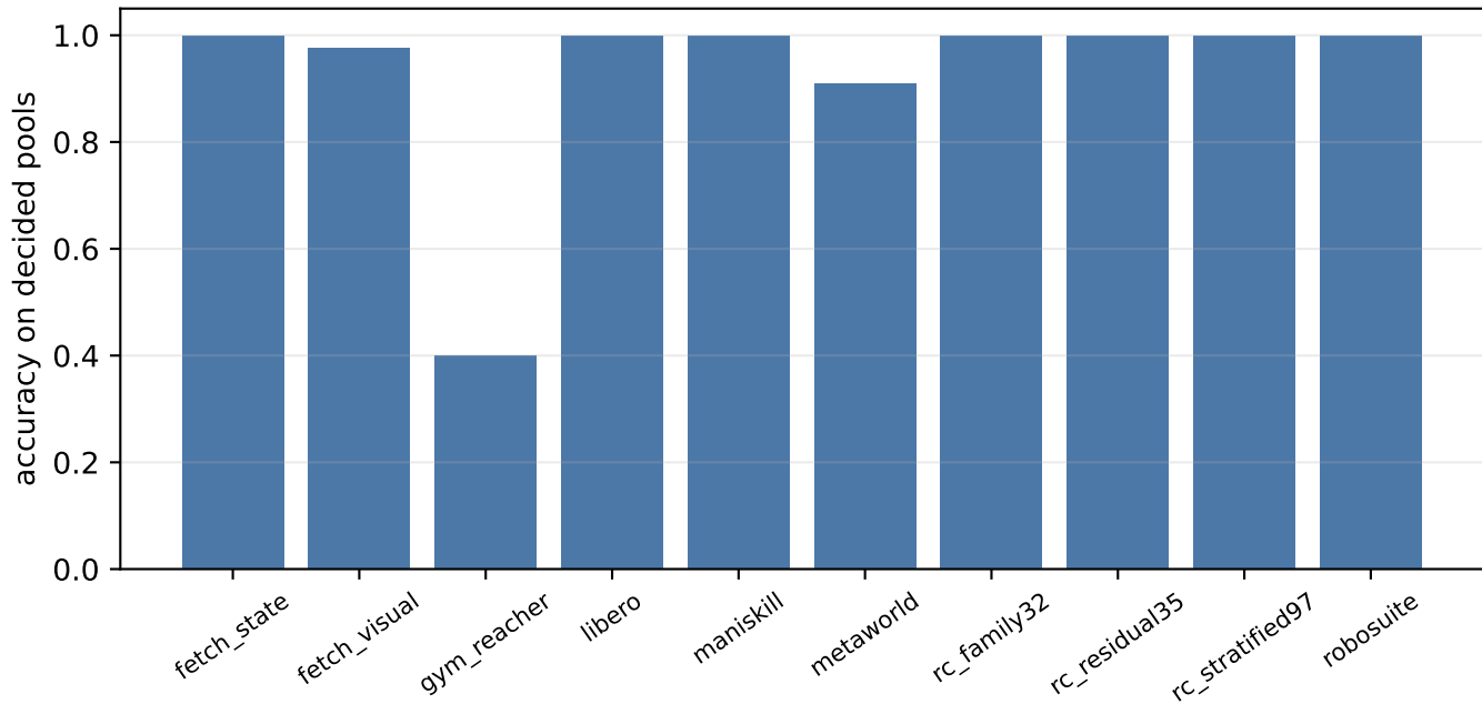
V6 leave-one-family-out decision accuracy
