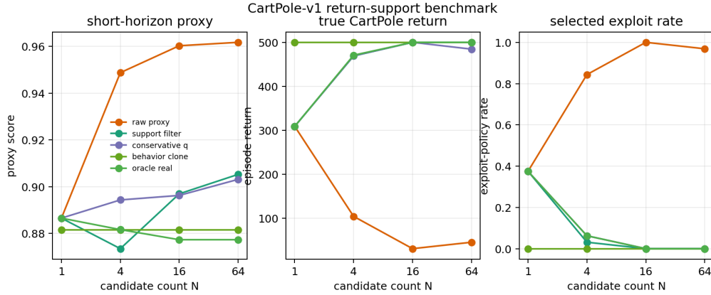
Figure 10: CartPole-v1 benchmark. Raw high- N proxy selection improves the short-horizon proxy while collapsing true episode return. Support-aware and conservative selectors give up a small amount of proxy score and recover true return.
