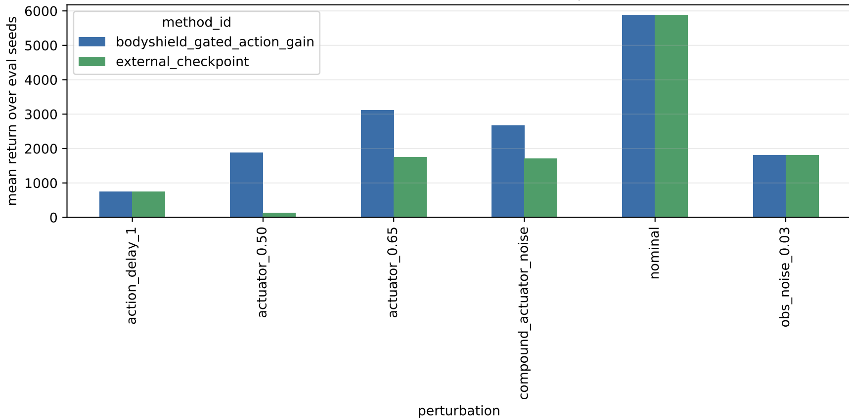
Public SB3 PPO HalfCheetah Checkpoint
