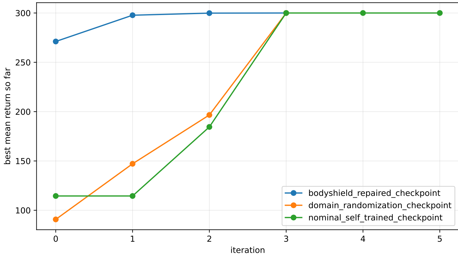
Self-Trained Public-Env CEM Training
