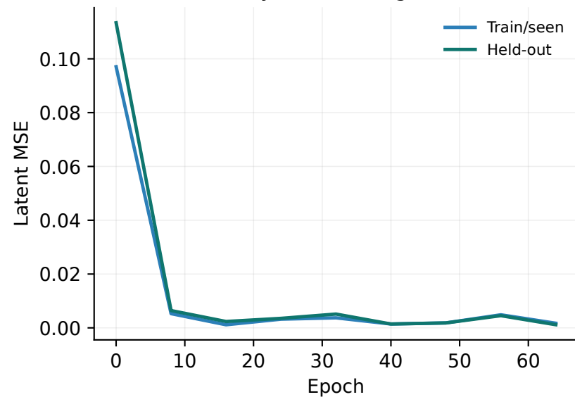
NumPy MLP training curve
