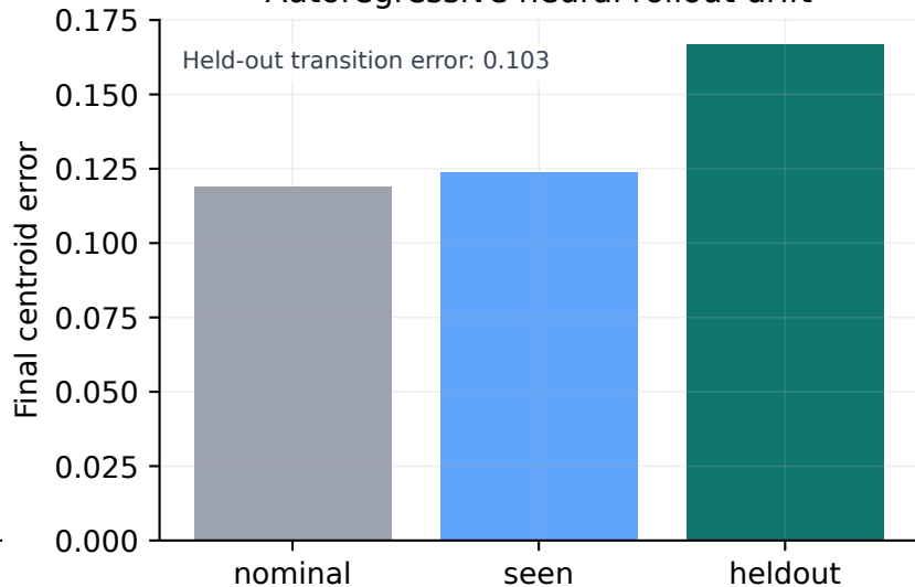
Autoregressive neural rollout drift
