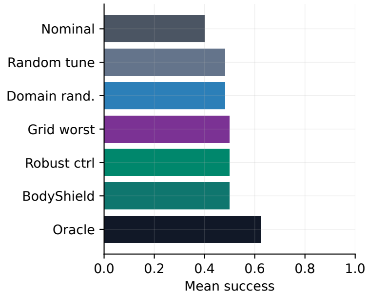
MuJoCo task-shaped probes
