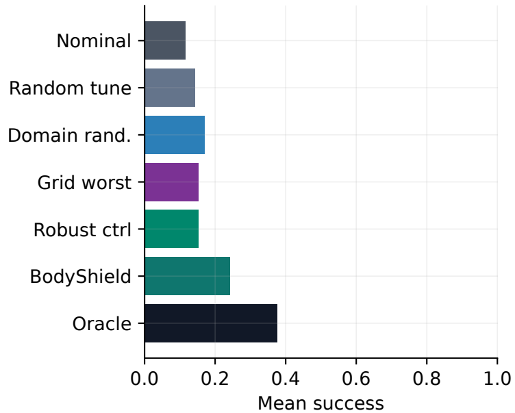
MuJoCo planar-effector probes
