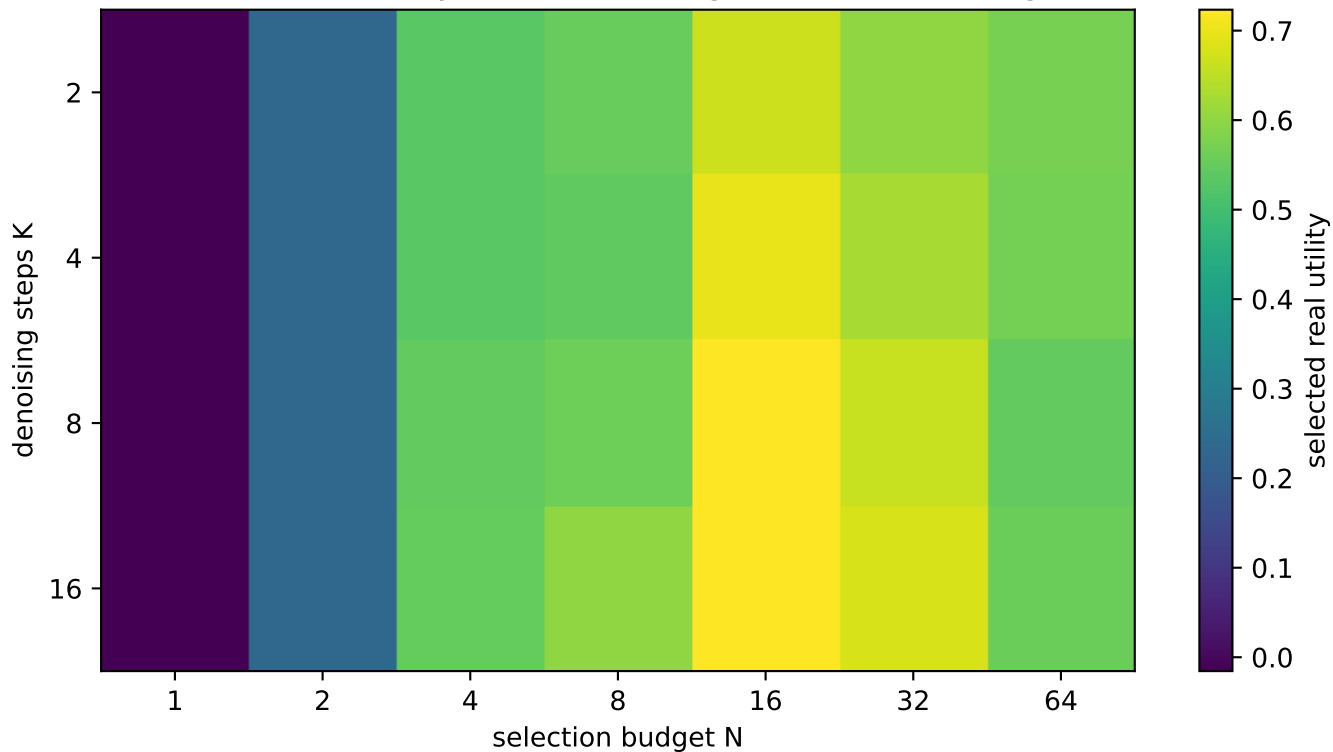
Selected real utility under denoising and selection budgets
