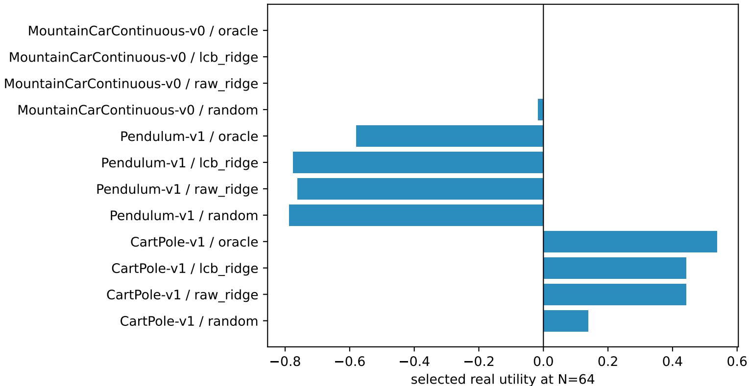
Gymnasium benchmark rollout-pool baselines
