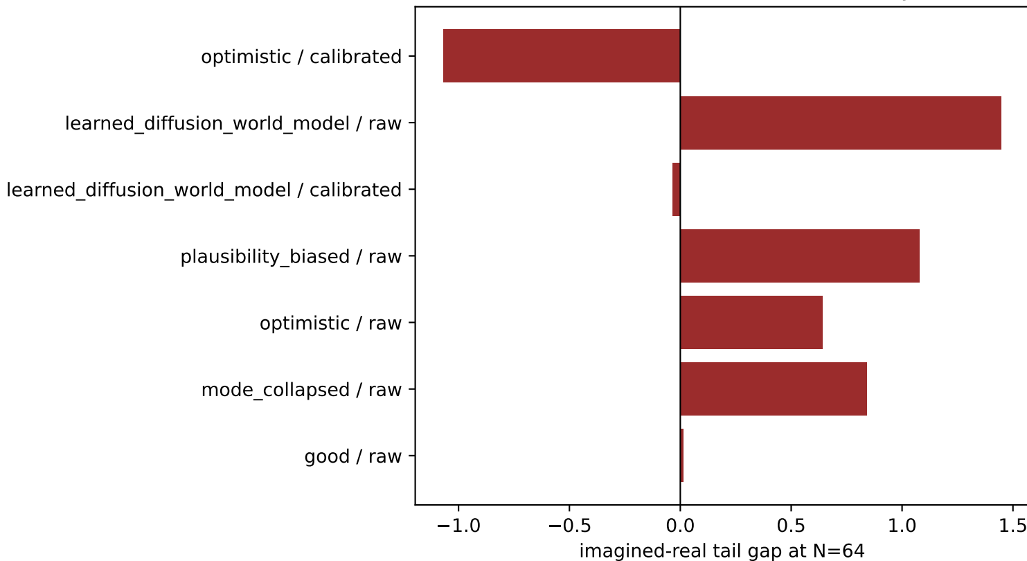
Selected-tail hallucination severity
