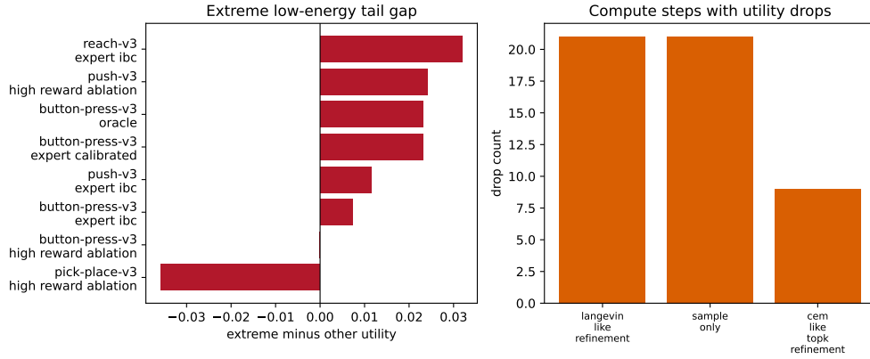
Figure 10: V4 adversarial stress summary. Left: worst extreme-low-energy reliability gaps. Right: compute-budget steps where extra optimization lowers measured utility. These rows force the paper to state when more inference is useful and when it is not.
