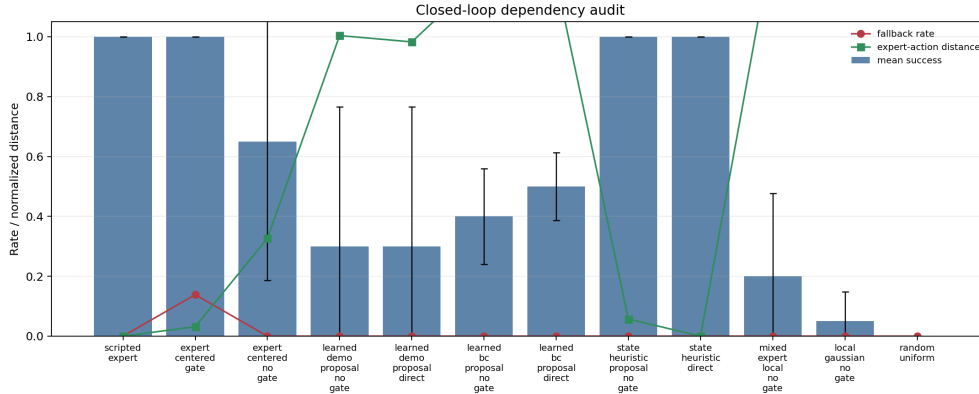
Figure 4: Closed-loop dependency audit. The figure separates expert-centered, learned-proposal, state-heuristic, random, and scripted variants so the supported claim does not overstate autonomy.
