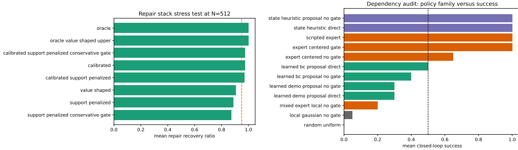
Figure 6: V3 repair and dependency audits. The main repair stack reaches mean recovery 0.972 and worst-case recovery 0.962 with 0 utility-degrading rows, while the closed-loop dependency audit keeps learned-proposal and state-heuristic outcomes separate.
