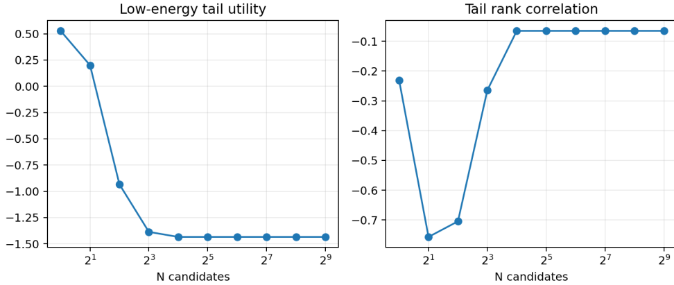
Figure 8: Tail rank and tail utility diagnostics.
