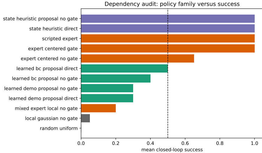
Figure 12: V3 closed-loop dependency audit. Expert-centered, learned-proposal, state-heuristic, random, and scripted variants are separated so the paper cannot silently claim autonomous learned-policy success.
