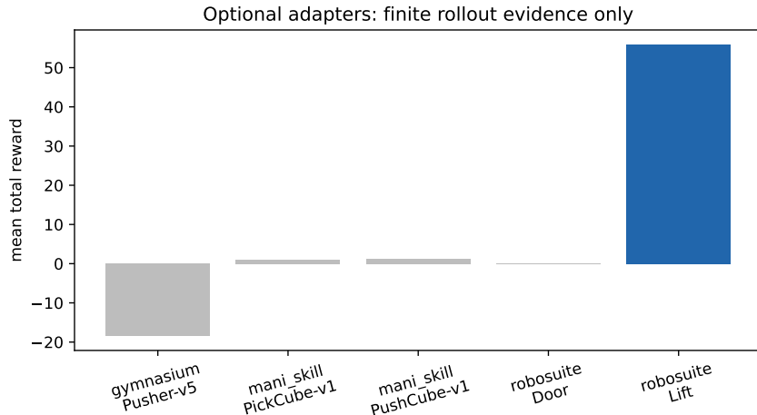
Figure 13: Optional adapter evidence. Rewards and success are reported as finite guarded rollout artifacts, not as real-robot or broad manipulation validation.
