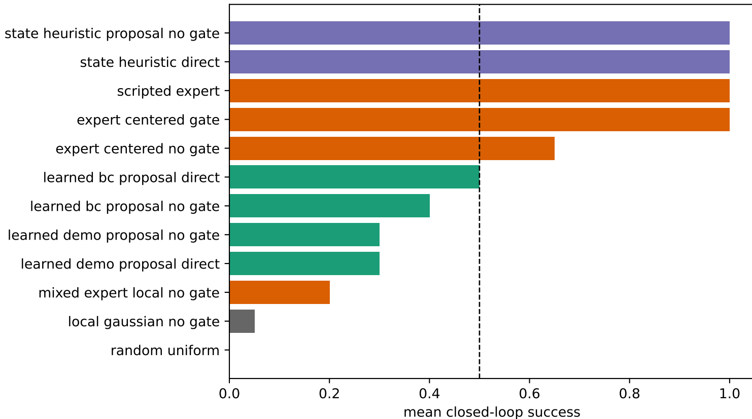
Dependency audit: policy family versus success
