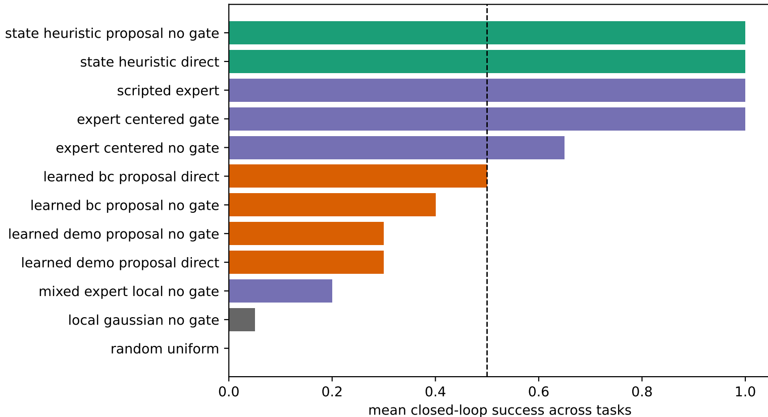
Claim gate: dependency and learned-policy boundaries
