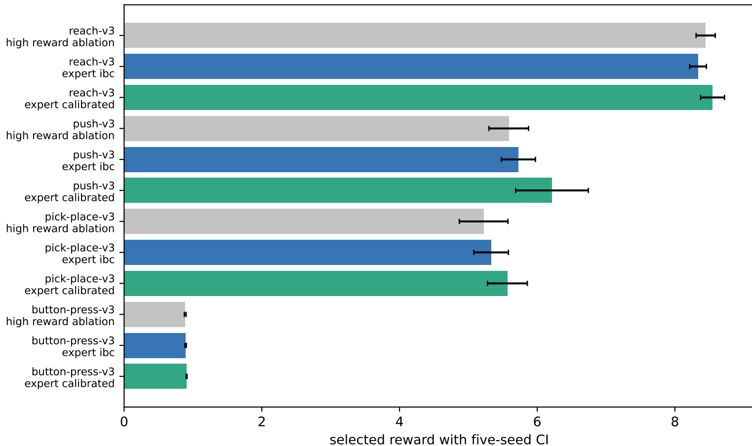
Meta-World selected-action baselines and controls
