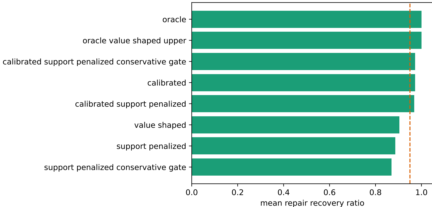
Repair stack stress test at N=512
