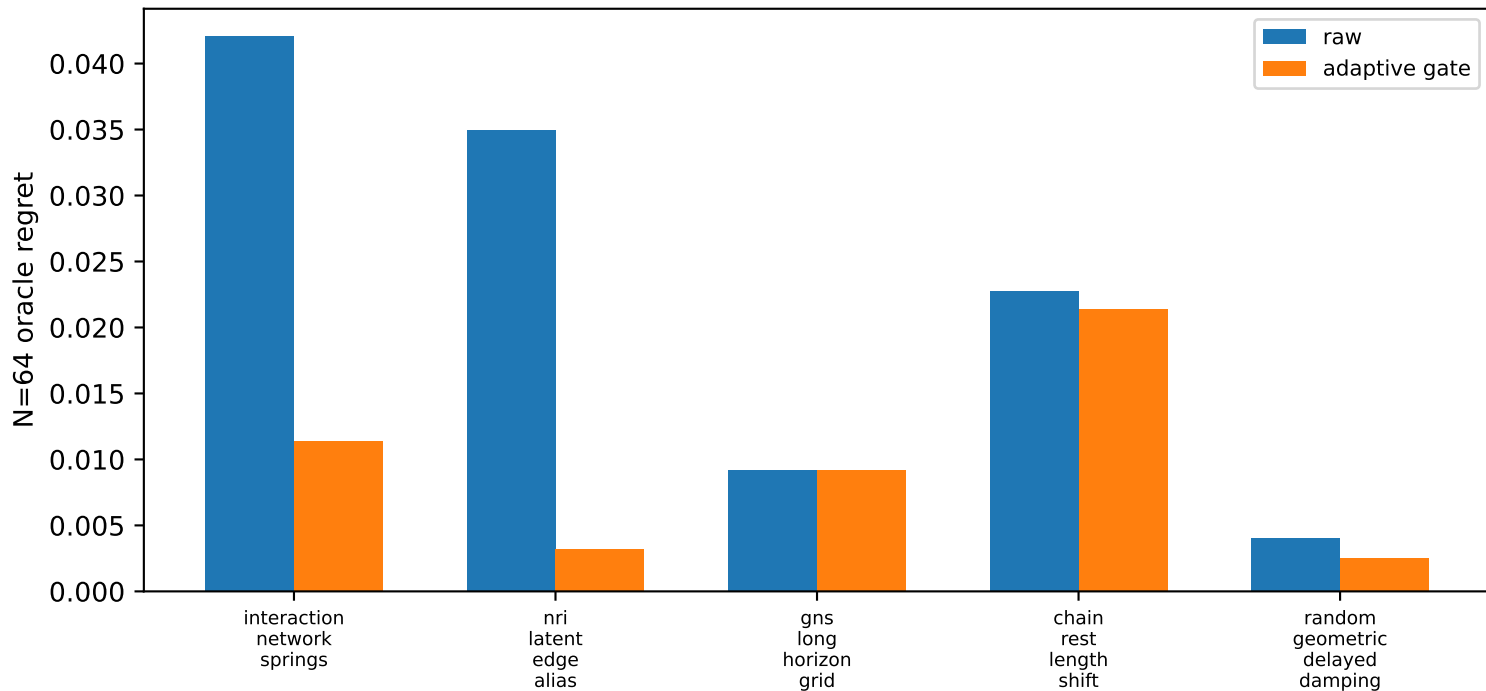
Recognized graph-dynamics protocol bridge
