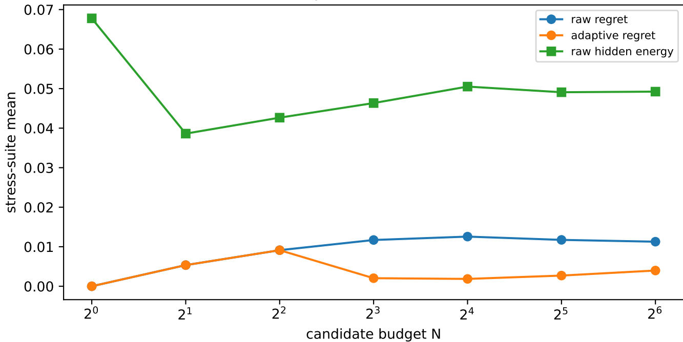
Compute frontier stress
