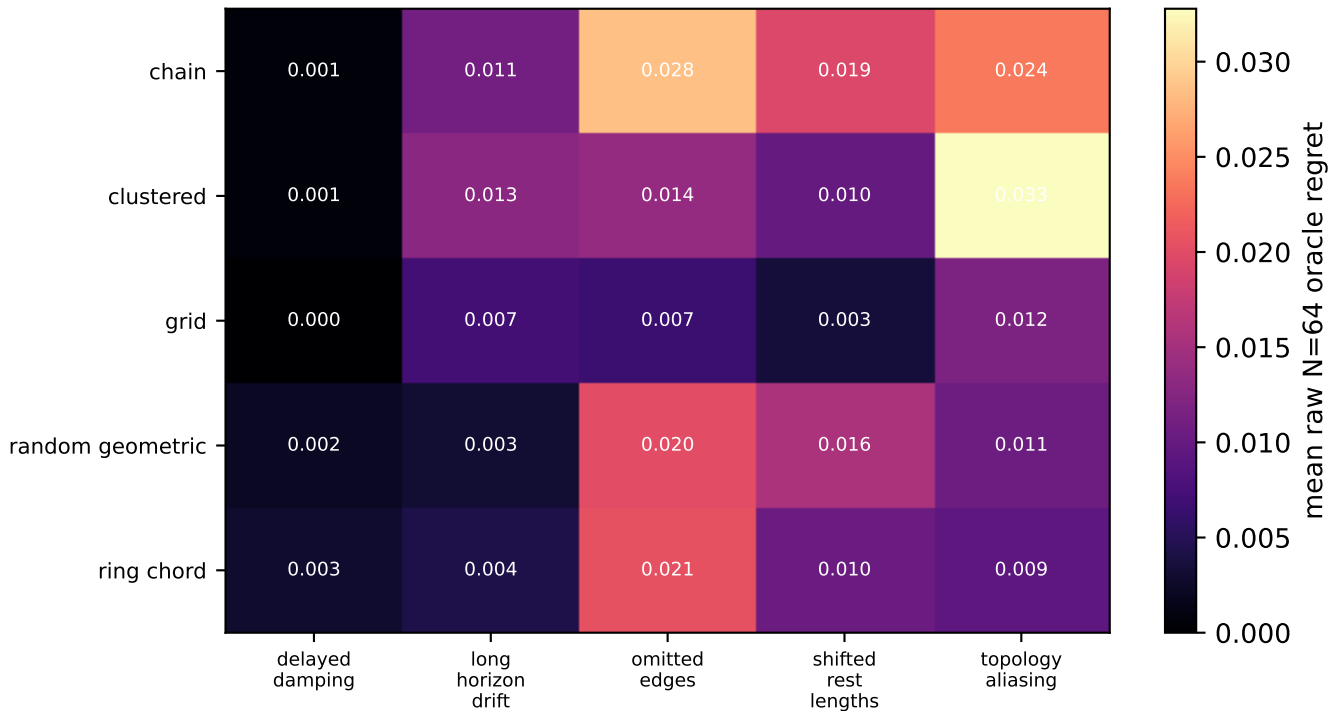
Constraint-shadow matrix
