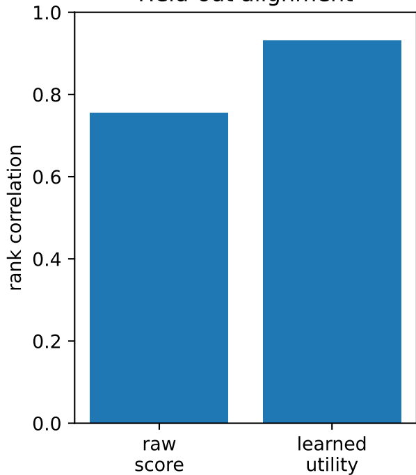
Held-out alignment
