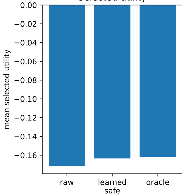
Selected utility
