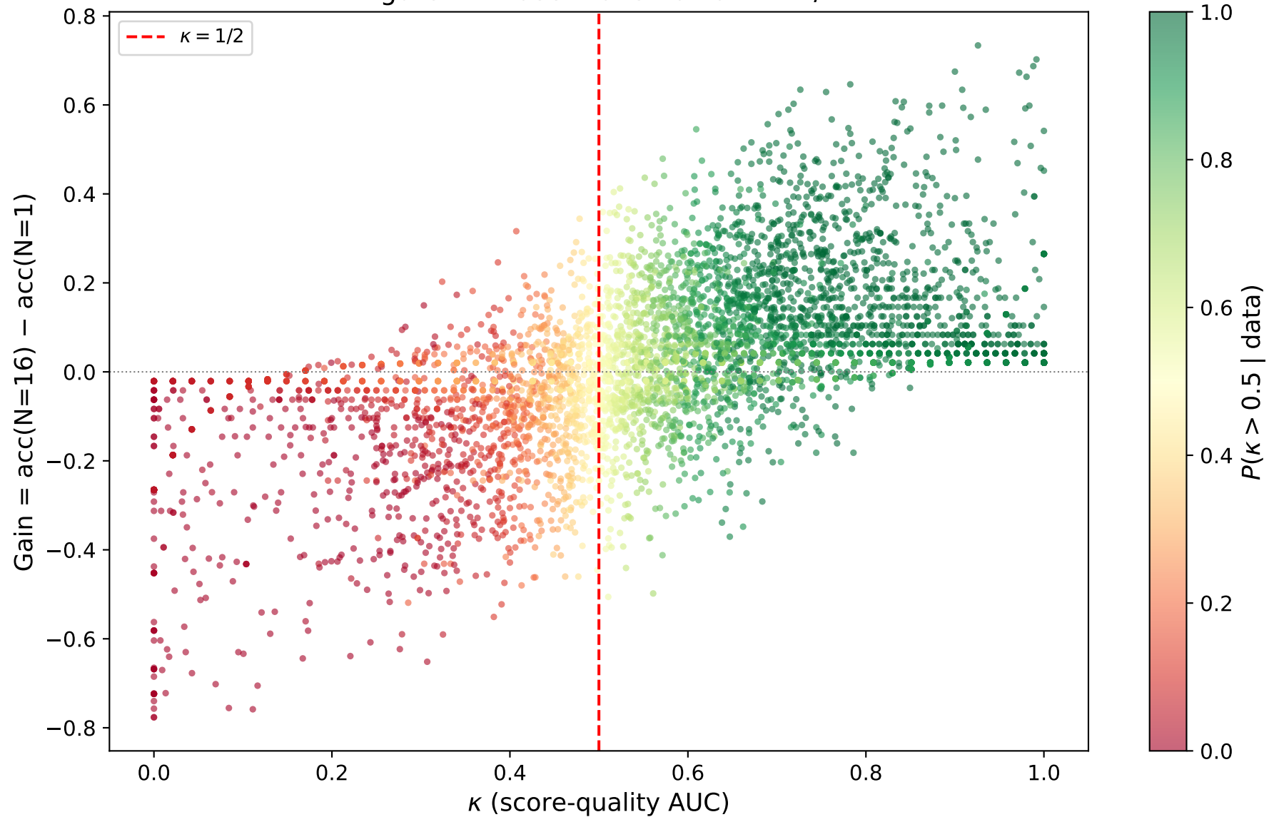
Figure 2: Phase Transition at \kappa = 1/2
