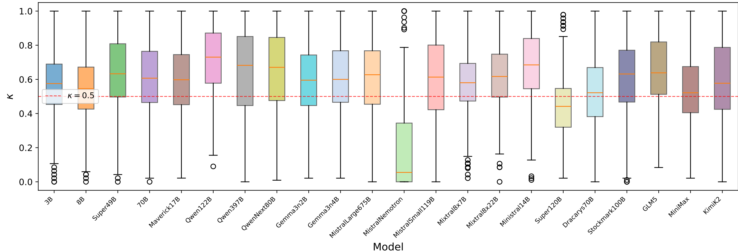
Figure 5: \kappa Distribution by Model
