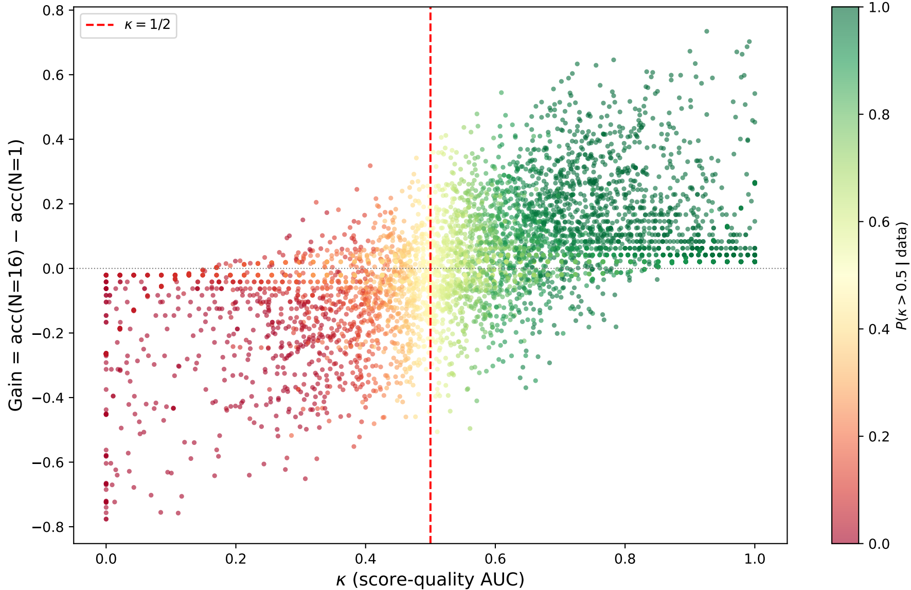
Phase Transition at \kappa = 1/2
