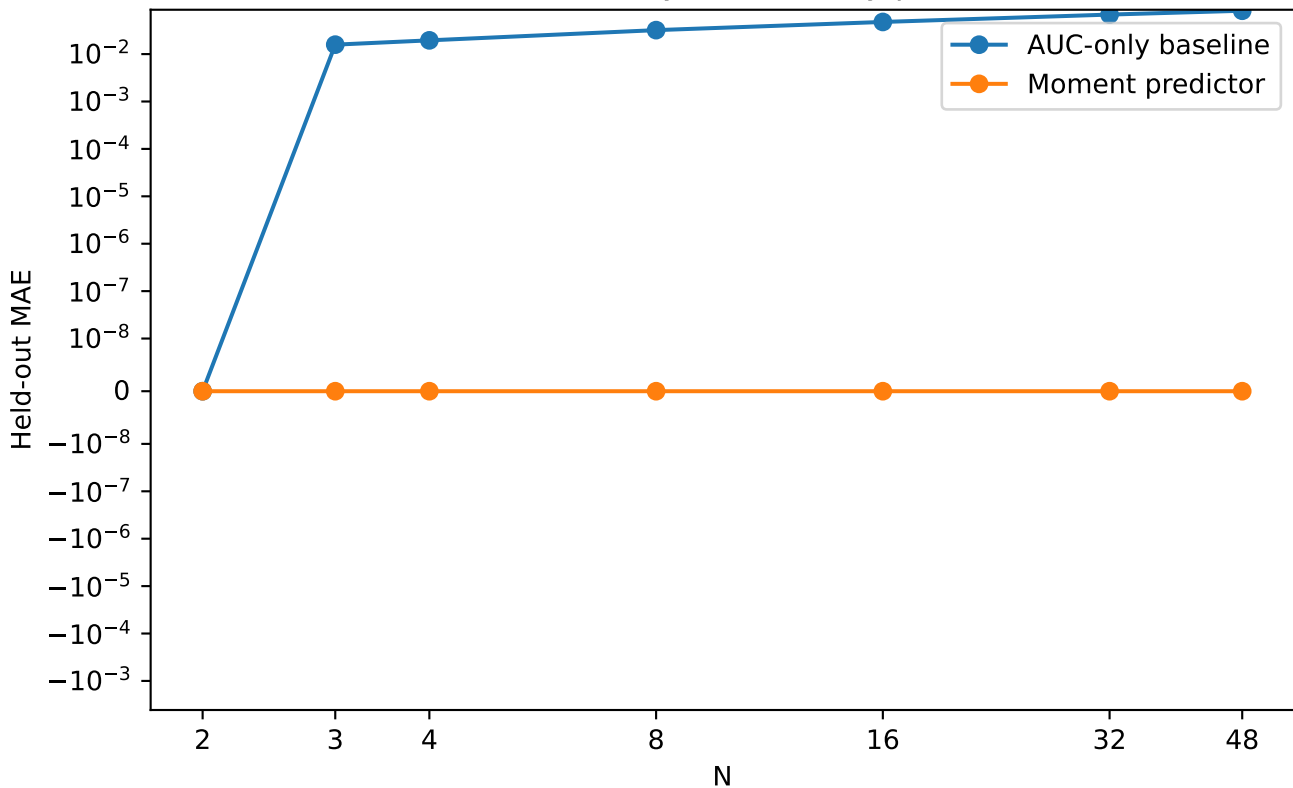
Moment hierarchy vs AUC-only prediction
