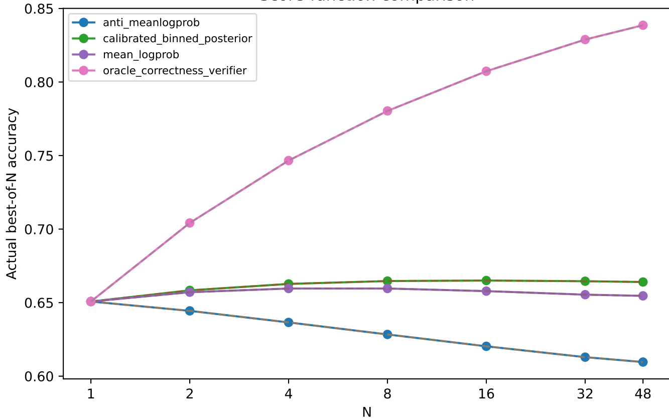
Score-function comparison
