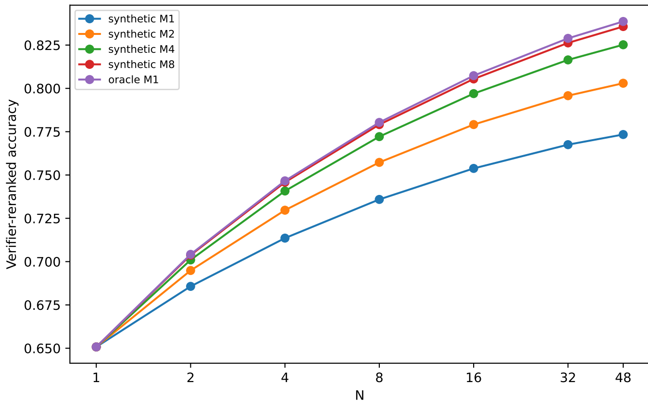
Verifier-score best-of-N extension
