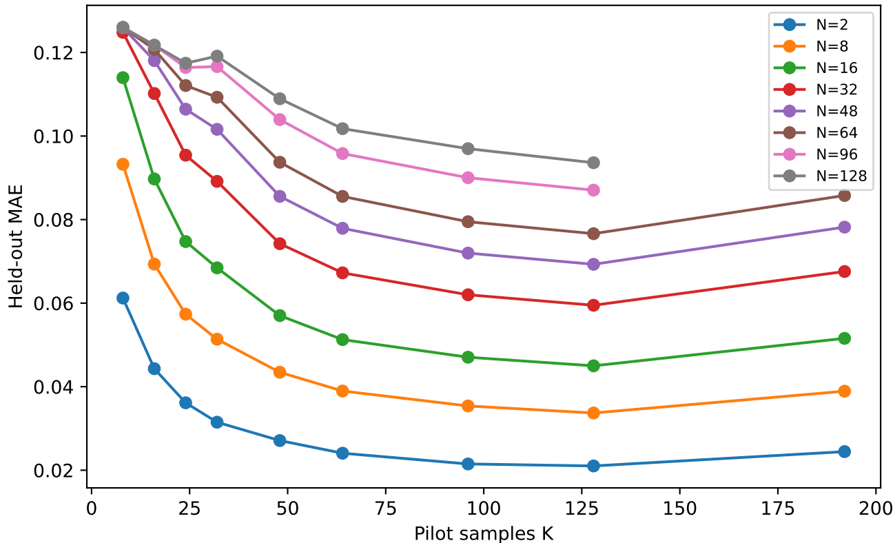
Expanded pilot sample-complexity (representative models)
