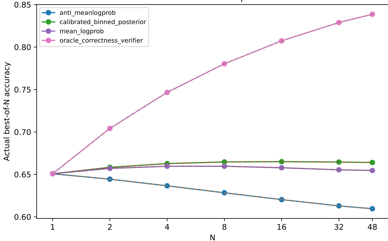
Score-function comparison
