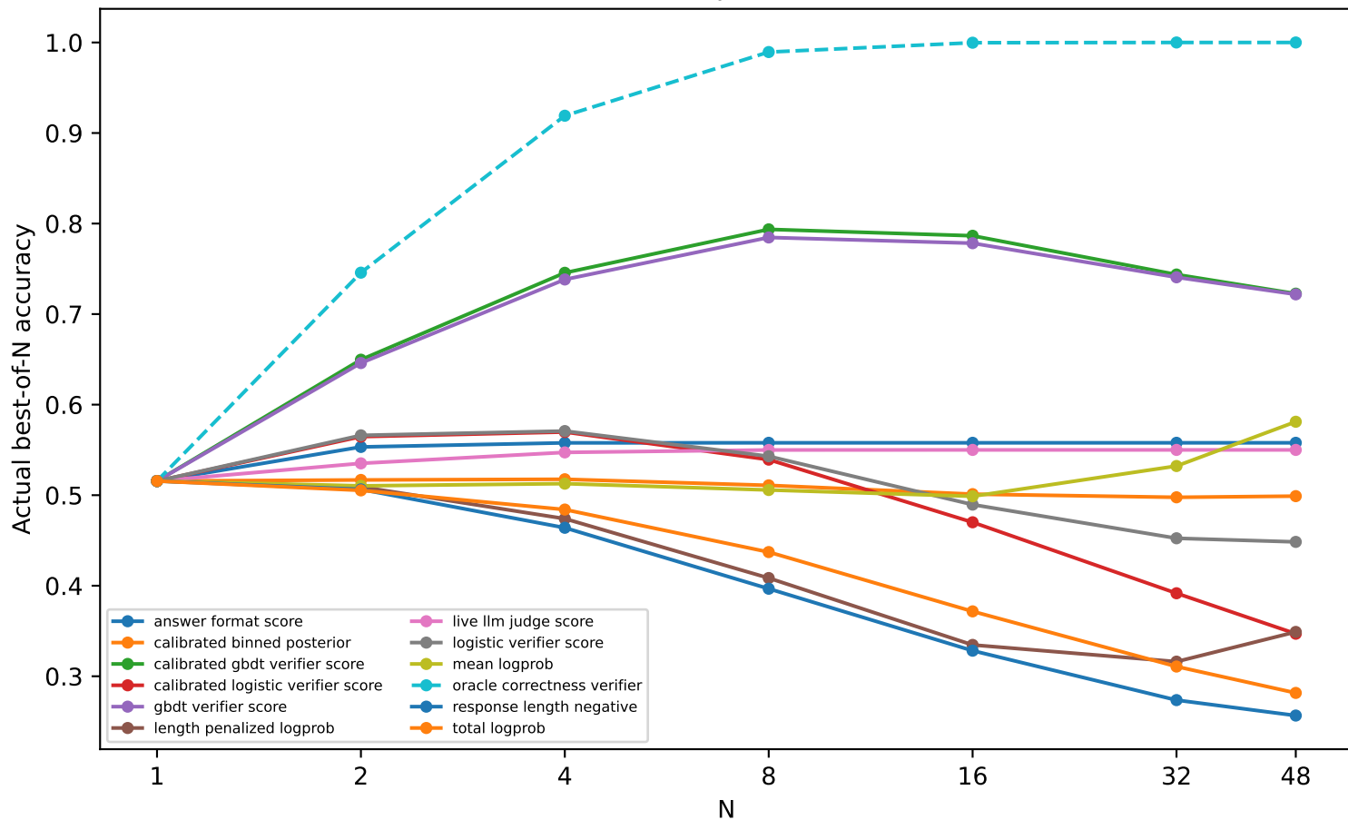
Score-function comparison (all features)
