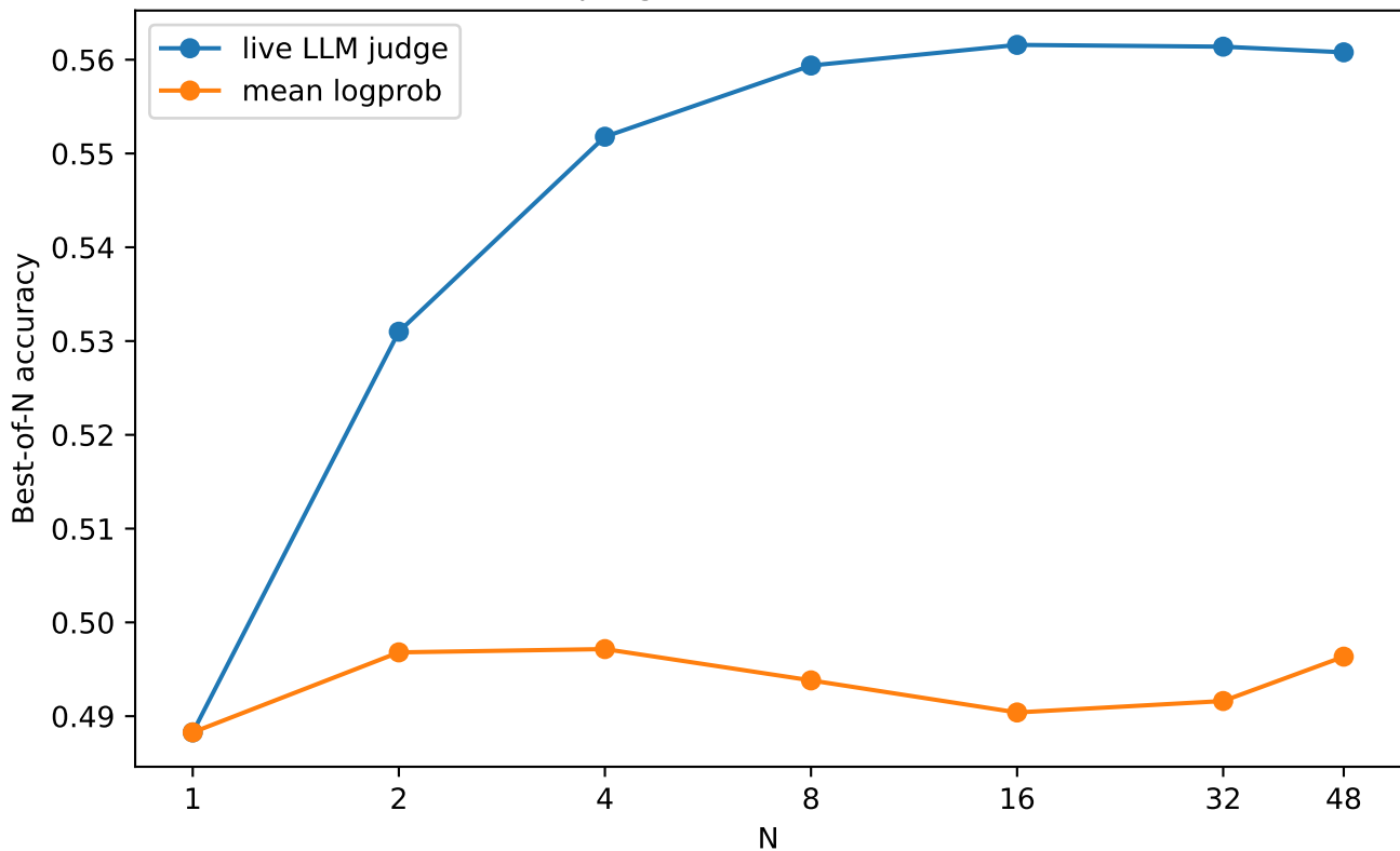
Live LLM judge score-function extension
