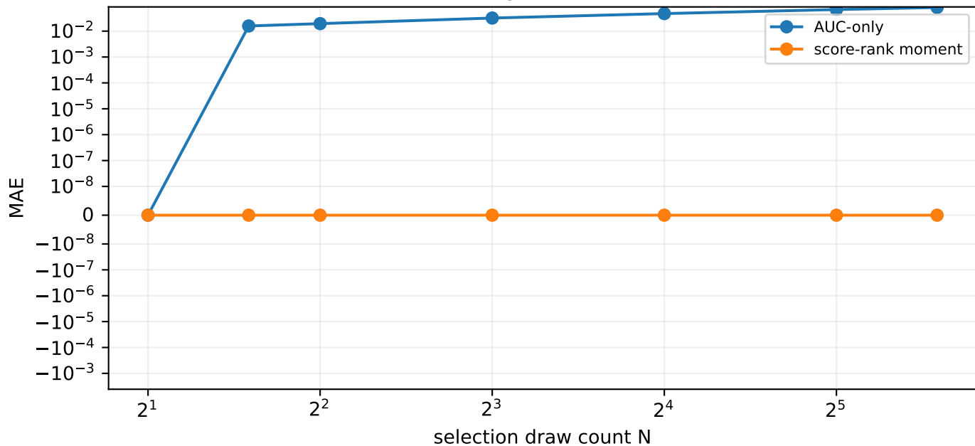
Pairwise AUC loses high-N score-rank information
