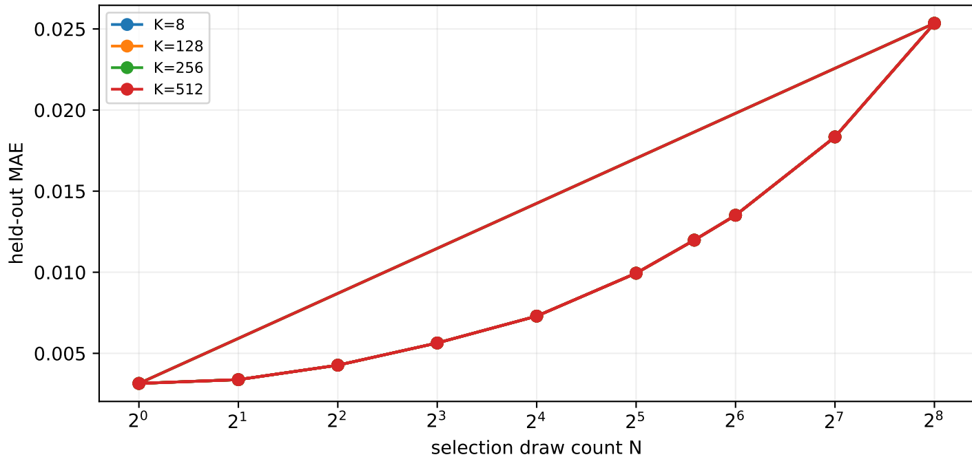
4096-depth held-out slice: error grows with N
