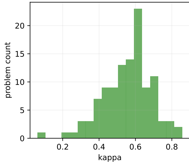
AUC/kappa distribution
