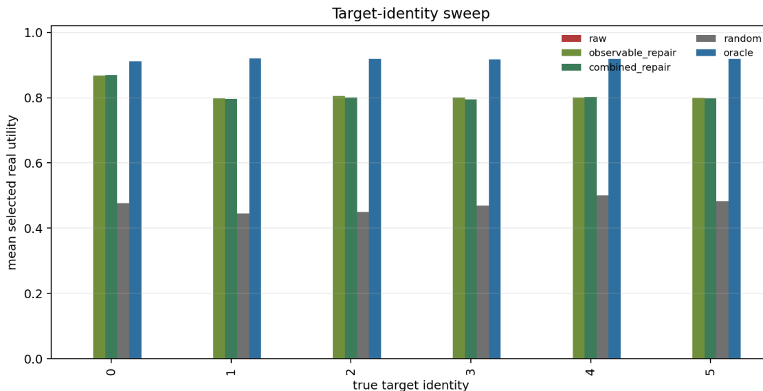
Figure 5: Target-identity sweep. The true target is varied over six identities, showing that the failure is not hard-coded to object zero.
