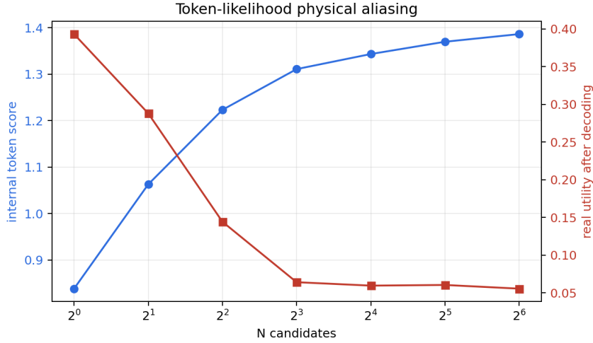
Figure 1: Raw Best-of- N selection amplifies token-likelihood physical aliasing. As N grows, selected token likelihood rises, but selected real utility falls because the high-score tail is dominated by aliased and physically invalid decoded futures.
