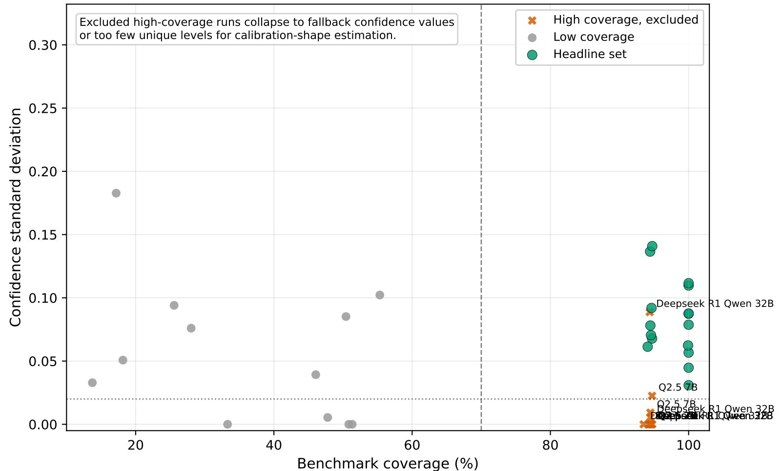
Confidence-quality audit of saved per-item traces
