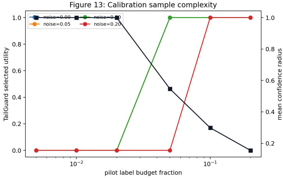
Figure 13: Pilot-label sample-complexity and selected-tail confidence radii.
