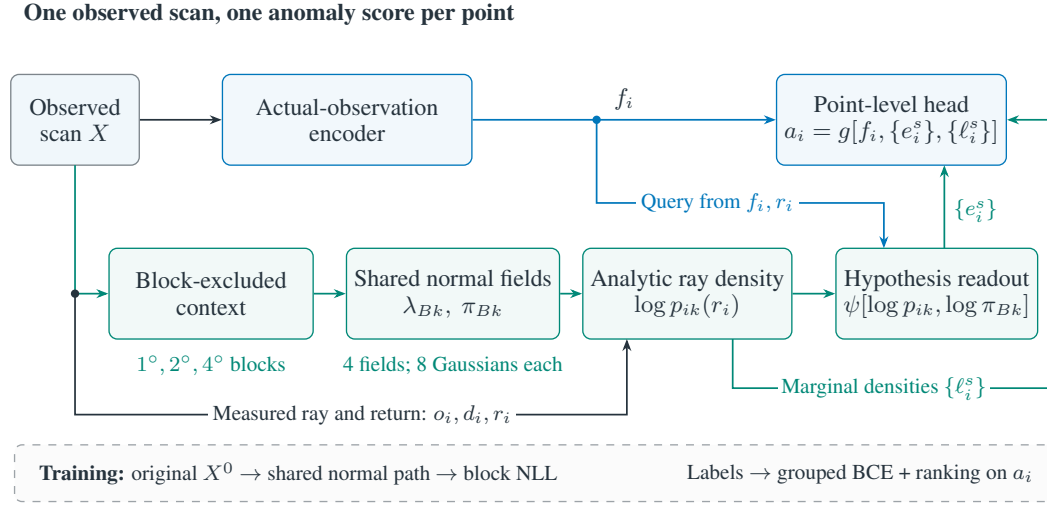
Figure 1: Contextual normal return fields. Block-excluded context predicts normal hypotheses, and analytic ray integration evaluates their support for each return. Hypothesis features and marginal log densities join actual-observation features in one point-level head. Normal-path parameters are shared across scales. During training, the unmodified companion X^0 supplies the separate block-likelihood objective.
