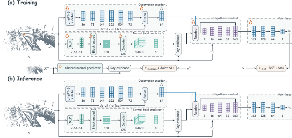
Figure 1: Contextual normal return fields. (a) Detection and original-scan likelihood jointly train the model using labels y and y^0 . The original companion uses the shared normal predictor and analytic ray evidence. (b) Inference outputs one anomaly score a_i per point. Solid boxes denote operations; grids depict feature tensors, with widths annotated. The observation encoder combines five encoder features, the final decoder feature, and point detail. Block embedding combines mean/max pooling with learned feature and position projections. The normal predictor excludes the target block, and decodes four hypotheses with two 128-dimensional attention layers. Each hypothesis contains eight Gaussian components; priors are predicted separately. Hypothesis readout includes query formation, evidence attention, and concatenation: 64 + 3 \times 32 + 3 = 163 channels. Dashed regions group computations; arrows show forward dependencies. Flames mark parameters optimized during source training, including the pretrained backbone; gray operations are analytic. Real nuScenes scenes share a viewpoint; orange marks auxiliary labels.
