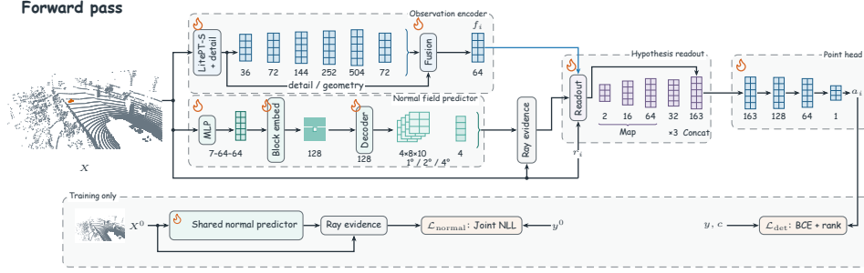
Figure 1: Contextual normal return fields. The forward path maps a scan X to pointwise anomaly scores a_i . Training adds the boxed detection and original-scan likelihood objectives; y and y^0 supply labels, and c identifies inserted normal controls. Inference uses the forward path alone. The observation encoder fuses all six backbone feature tensors with point detail and input geometry. Block embedding combines mean/max pooling with learned feature and position projections. The normal predictor excludes the target block and decodes four hypotheses with two 128-dimensional attention layers, sharing parameters across 1^\circ , 2^\circ , and 4^\circ grids. Each hypothesis contains eight Gaussian components; four prior weights are predicted separately. Ray evidence computes conditional return densities and carries the priors to the readout. Within the composite readout, grids annotate the 2–16–64 hypothesis map, a 32-dimensional read per scale, and concatenation to 64 + 3 \times 32 + 3 = 163 channels. The measured range r_i helps form the readout query. Dashed regions group computations; arrows show forward dependencies. Flames mark parameters optimized during source training, including the pretrained backbone. Gray operations are analytic and differentiable. Real nuScenes scenes share a viewpoint; orange marks auxiliary labels.
