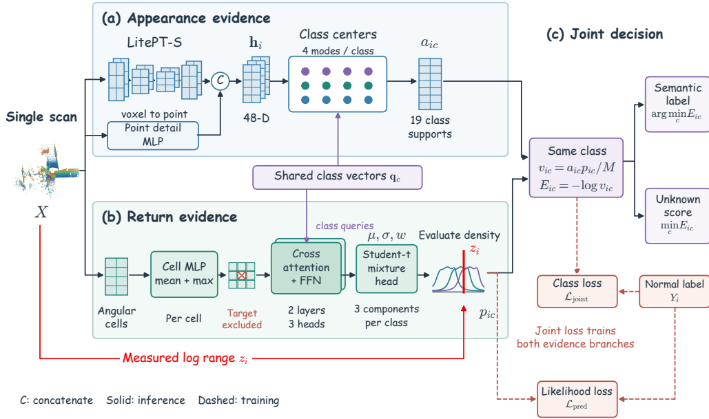
Figure 1: SERVE architecture. The full-scan branch combines voxel features with point details and projects them to a 48-dimensional embedding. Shared class vectors organize appearance centers and query independently encoded surrounding cells. Within the prediction branch, target exclusion precedes cross-cell attention; the actual target range enters only the subsequent density evaluation. Evidence combines within each class before semantic labeling and unknown scoring. Dashed paths show the joint classification and predictive likelihood objectives; auxiliary losses are specified in Equation (11). The input is a real LiDAR scan, colored by height and cropped to 2.5–35 m range and −3–8 m height. Density curves are schematic.
